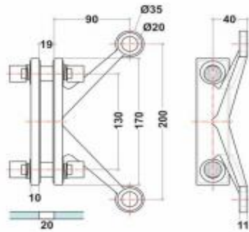
> ISF - 2 (316 Grade) Finish Satin, Glossy Type 2 Way Fin Type Spider
