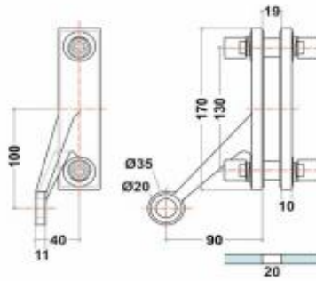
ISF - 4 (316 Grade) Finish Satin, Glossy Type 1 Way Fin Type Spider 90°
