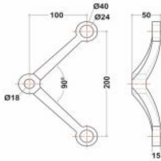
> ISF - 8 (316 Grade) Finish Satin, Glossy Type 3 Way Point Type Spider
