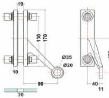
ISF - 5 (316 Grade) Finish Satin, Glossy Type 1 Way Fin Type Spider 45° Right Side
